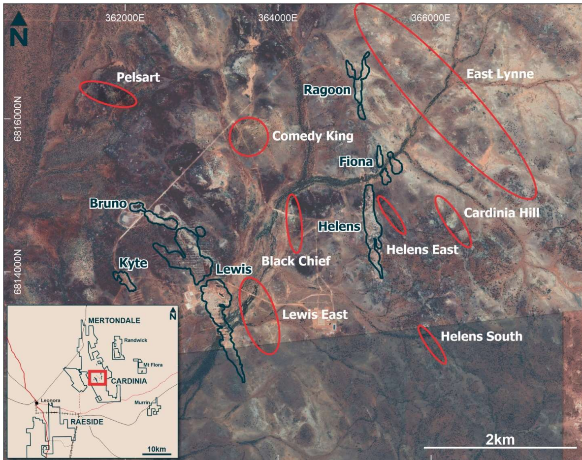
Figure A2 – Kin's Cardinia Gold Project showing existing deposits and exploration targets in the Phase 3 drilling program
