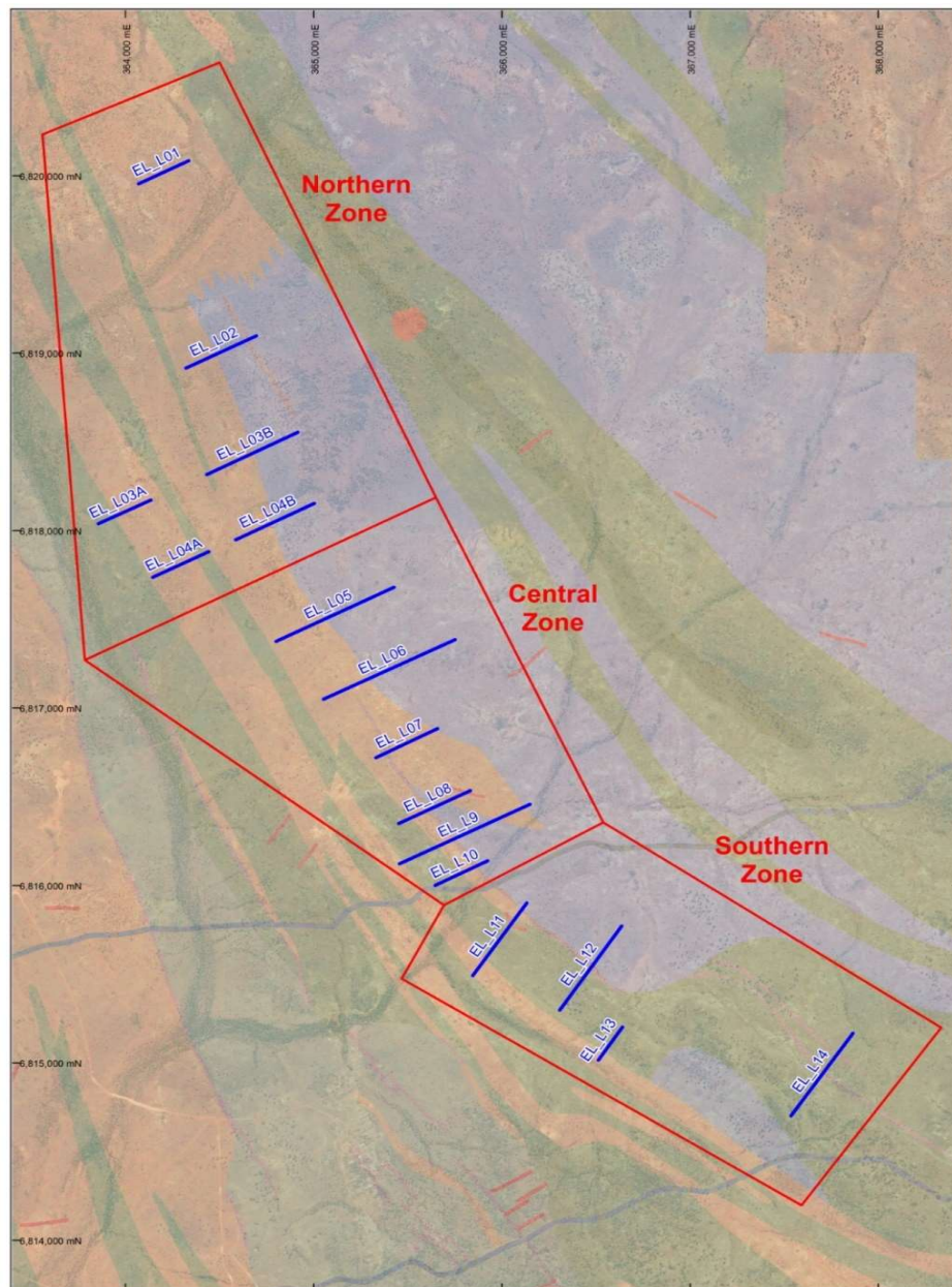
Figure 1: Location of the East Lynne AC drilling program. Results for Lines 5 and 6 within the Central Zone are reported in this announcement
