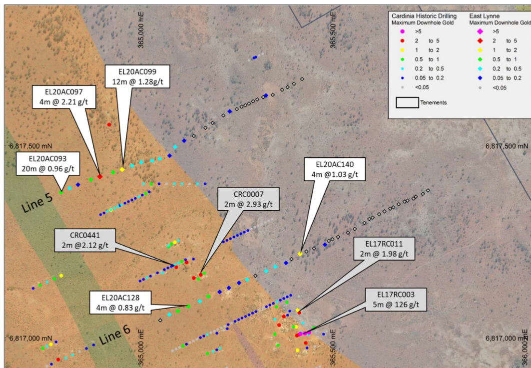
Figure 2: Location of the East Lynne AC drilling program. Results for Line 5 and Line 6 are reported in this announcement and illustrated with white shaded labels. Historical RC results are illustrated with grey shaded labels
