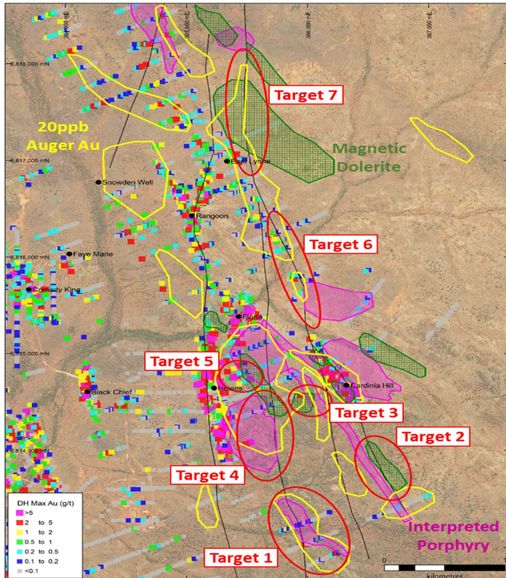
Figure 2. Eastern Corridor Targets 1 to 7 generated by the recent Gravity survey and integrated with multi-element soil geochemistry and historical and recent drilling data.
