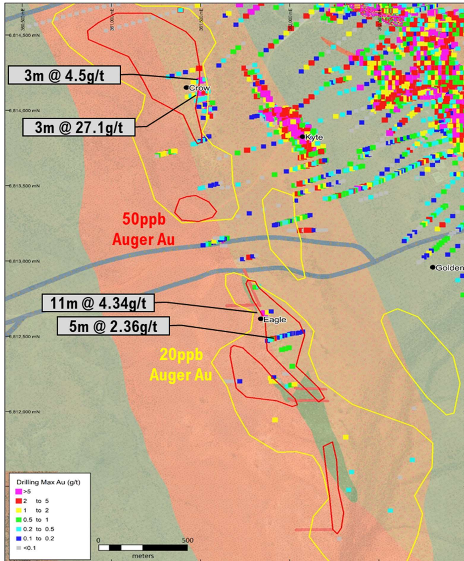
Figure 4. Eagle Target illustrating the extensive 6km by 1.0km soil geochemical anomaly and the historical drilling results along the eastern edge of the anomaly. The Kyte and Bruno Lewis deposit locations are shown as intense drill-hole locations in the upper centre and upper right of the figure.
