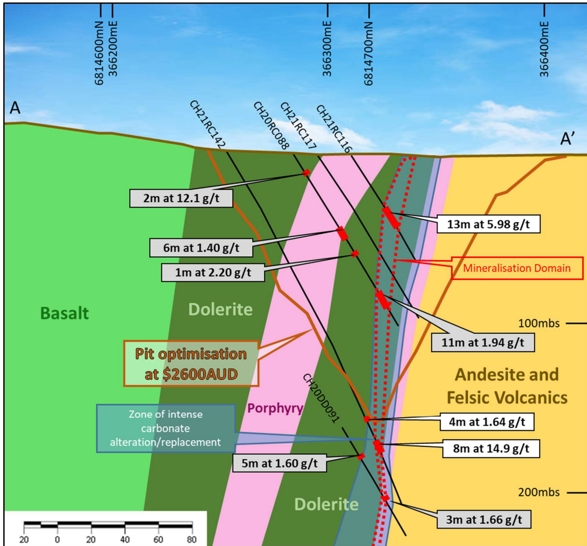
Figure 2: Location of the Cardinia Hill RC and DD results in the Southern Shoot drilling (Figure 1 A-A'). True width is approximately 70% of down-hole intersection. Note: CH21RC117 has been drilled and is awaiting results. New results shown in white labels, previous results grey labels.
