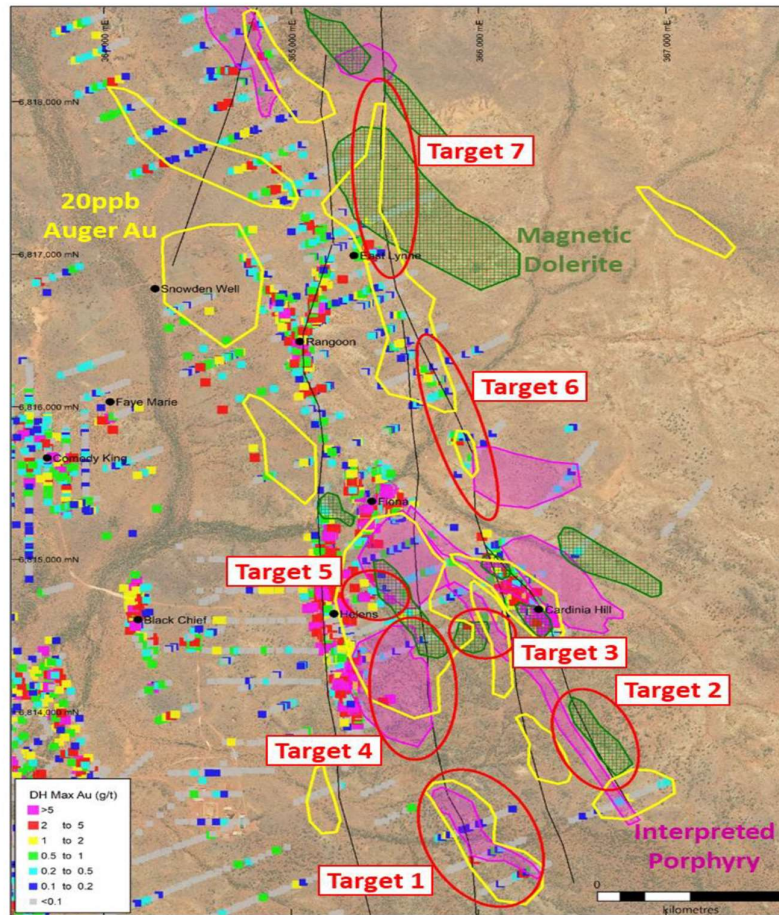
Figure 4. Location of the Eastern Corridor mineralised system in relation to the new geological interpretation based on the recent Gravity survey data. The Helens and Cardinia Hill deposits and other Eastern Corridor targets (Targets 1-7) follow established fault positions, interpreted intrusion contacts and are confirmed by historical workings and shallow AC drilling.
