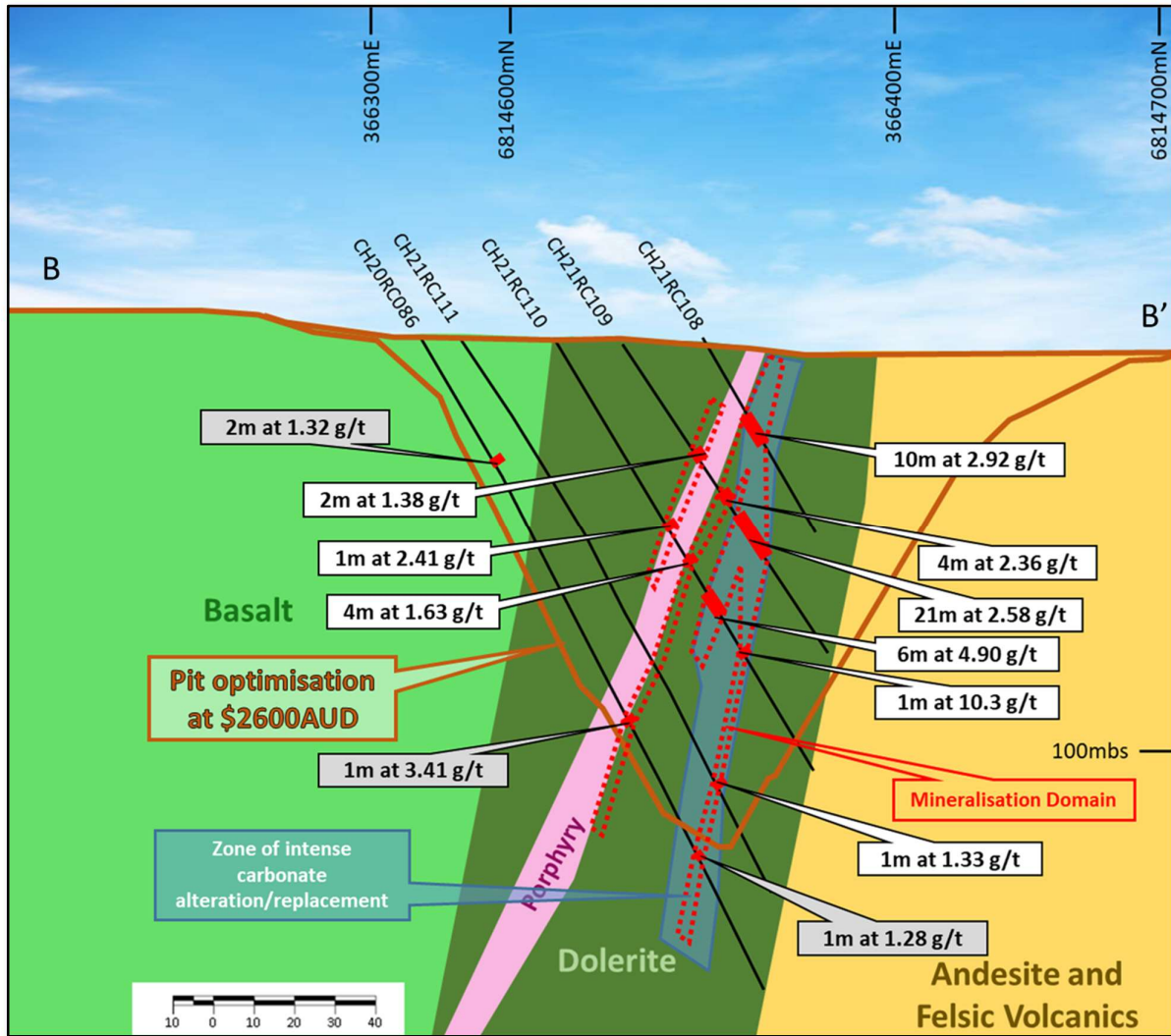
Figure 3: Location of the Cardinia Hill RC and DD results in the Southern Shoot drilling (Figure 1 B-B'). True width is approximately 70% of down-hole intersection. New results shown in white labels, previous results grey labels.
