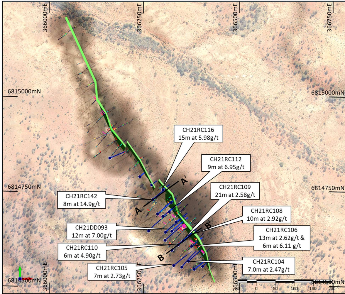
Figure 1: Location of the Cardinia Hill RC and DD Resource Definition drilling program. Aerial photo draped over optimised pit wireframe. The Cardinia Hill mineralisation extends for more than 700m and remains open at depth and to the north.
