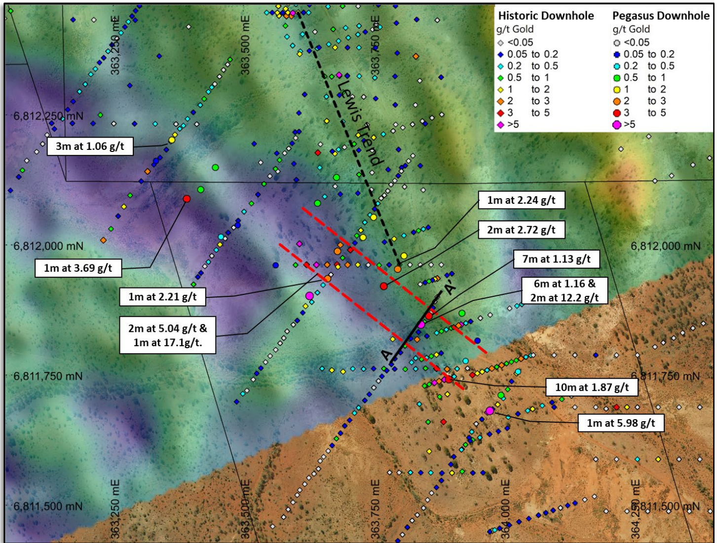
Figure 2: Pegasus RC drilling results over detailed gravity map. Recent RC results in white labels. Pegasus RC and AC drilling defines a zone containing several mineralised lodes trending NW-SE for over 600m of strike that lies within a significant gravity low.
