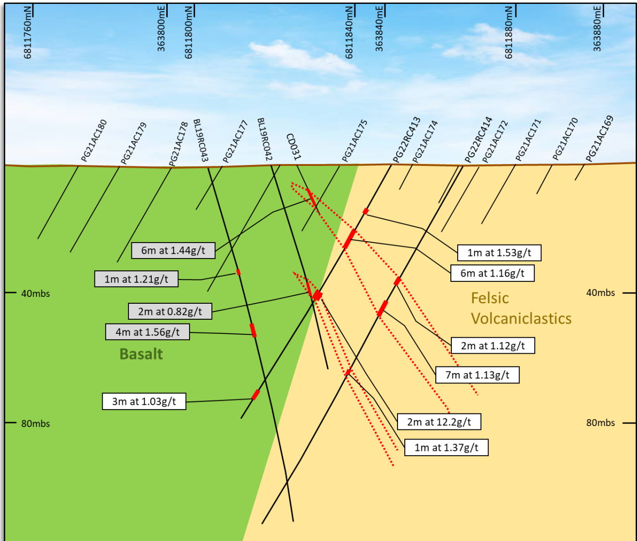
Figure 3: Pegasus RC drilling results cross section A-A' illustrating two zones of east dipping, gold mineralisation within Felsic Volcaniclastic rocks. Recent RC results in white labels, historical drilling results in grey labels. High grade zones correspond to east dipping zones of increased sulphide mineralisation.
