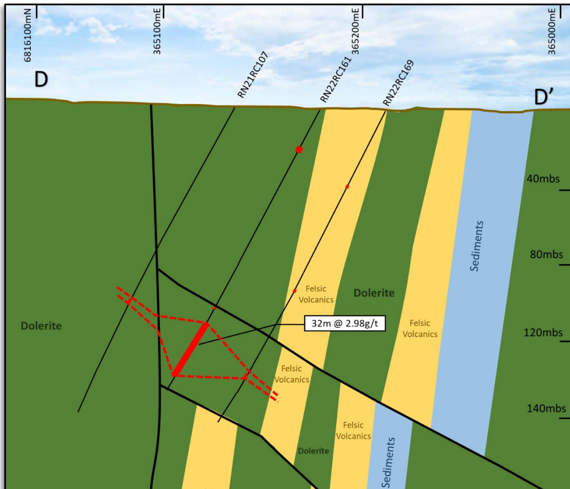
Figure 8: Rangoon drill hole cross section D-D' indicating the position of new zones of mineralisation. Section D-D' shows a zone of high-grade steep east ore adjacent to the Helens Fault position. New drill results in white labels.
