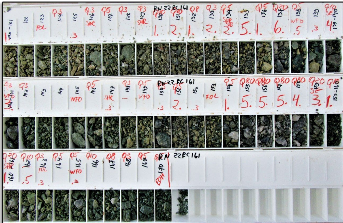
Figure 4: RC Chip tray RN22RC161 - 120m to 170m. Gold Mineralisation - 32m at 2.98g/t Au from 129m to 161m including 12m at 5.62g/t Au from 129m and 12m at 2.25g/t Au from 149m. Downhole metres shown in black. Logging shown in red - Q10 corresponds to estimated 10% quartz. Red numbers above rock chips (generally 1 to 6) correspond to logged sulphide % of the mineralised zone. Higher logged sulphide % correlates strongly to higher gold grades.
