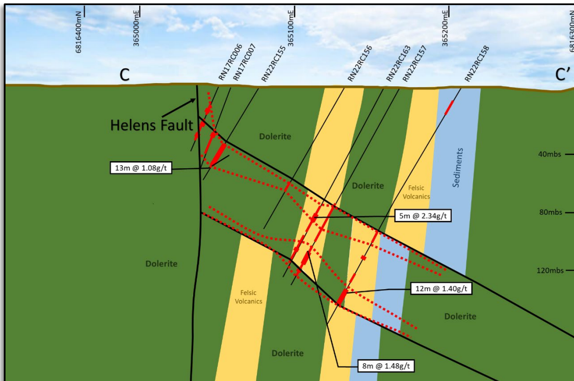
Figure 7: Rangoon drill hole cross section C-C' indicating the position of new zones of mineralisation dipping shallowly to the east. Section C-C' shows a near vertical near surface zone adjacent to the Helens Fault position and two high-grade shallow east dipping zones. New drill results in white labels, historical drill results in grey labels. True width is approximately 100% of drill intersections.
