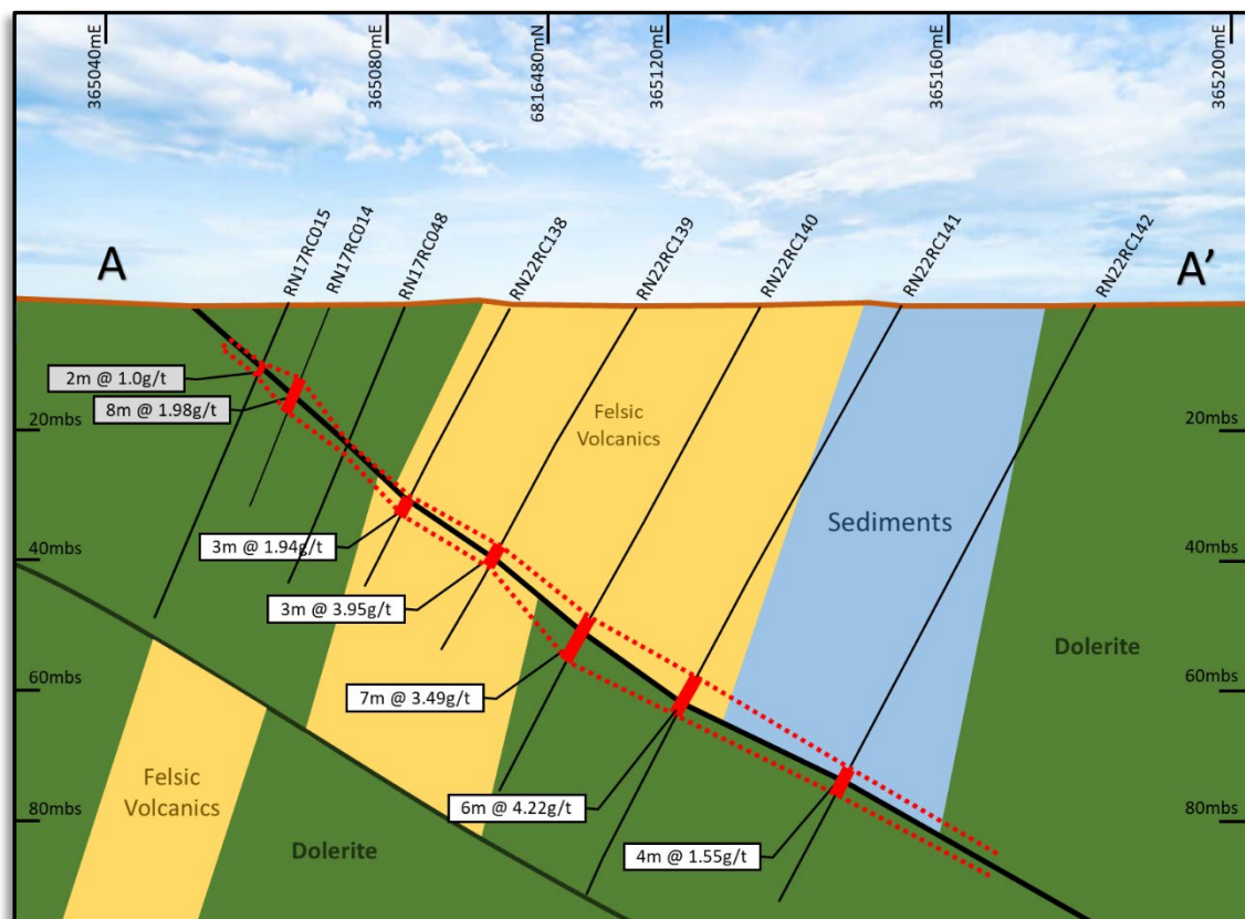
Figure 5: Rangoon drill hole cross section A-A' indicating the position of new zones of mineralisation dipping shallowly to the east. Section A-A' shows a single high-grade zone dipping shallowly to the east. Drill holes require extension to test the interpreted position of the lower structure. New drill results in white labels, historical drill results in grey labels. True width is approximately 100% of drill intersections.
